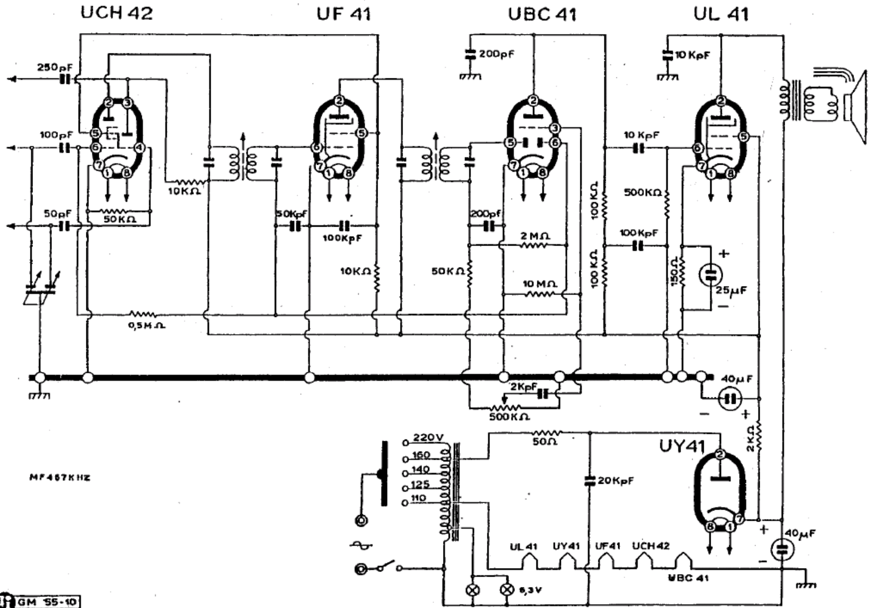
ELECTA RADIO - Mod. 520/B
